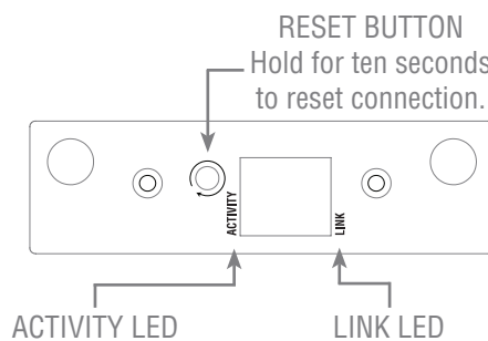
BlueBOLT-CV1 Network Interface Card Panel.
