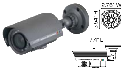
CVC5715DNV CVC5715DNVW (White Housing) 4-9mm Auto Iris Varifocal Lens
